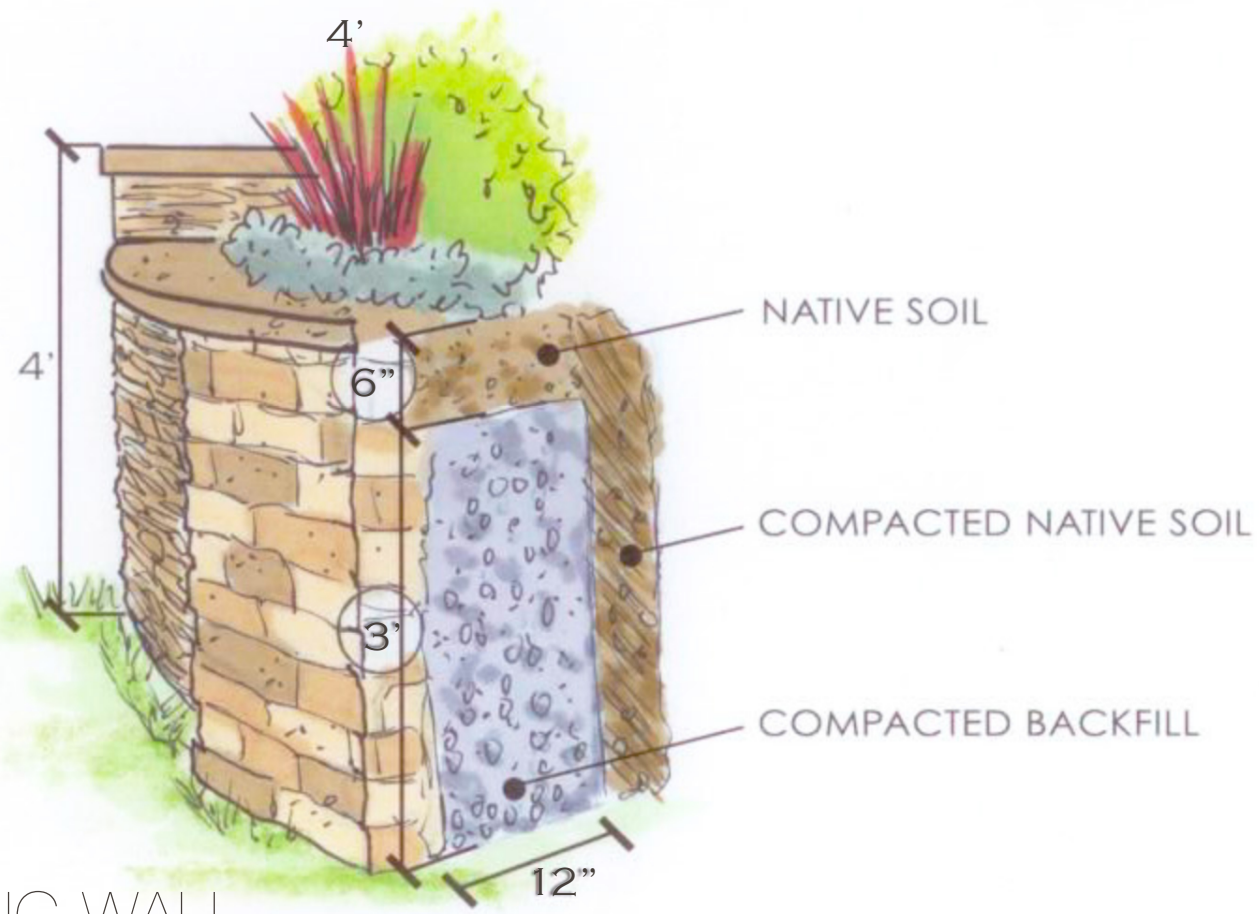
RETAINING WALL
